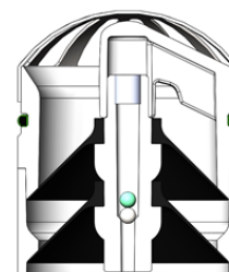
Unique Double-Skirt Silicone Valve System
