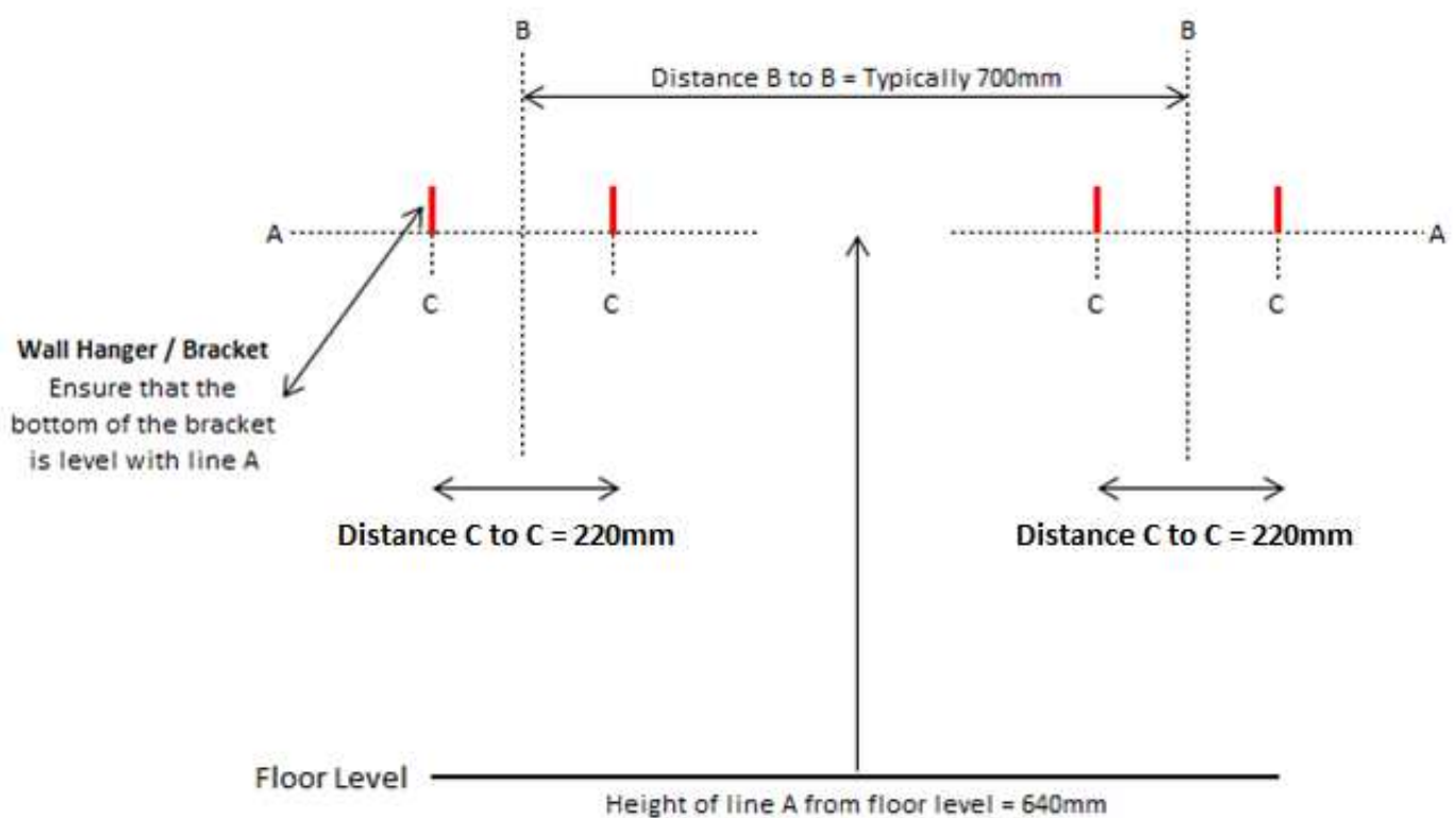
Installation diagram for KAROO Waterless Urinals
