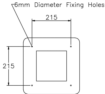
Base Fixing Details
