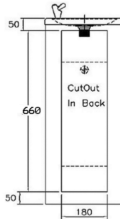
Rear View (Open Back Junior Version)
