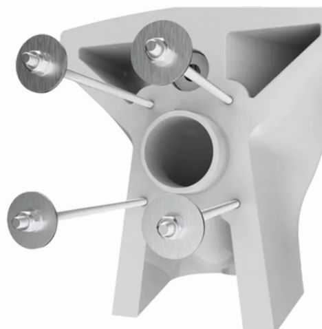
Rear View Showing 4x M10 x 300mm Wall Fixing Tie Rods
